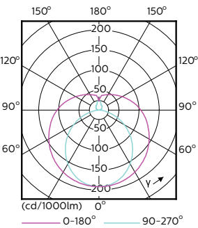
LEDtube 1200mm 17W G13 2100lm
